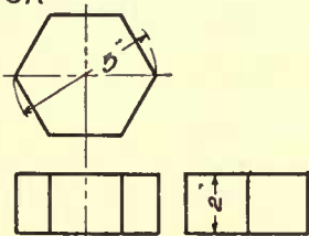
WORKING DRAWING
